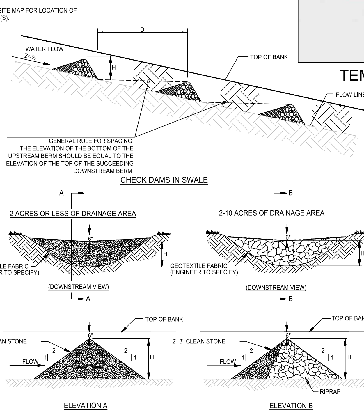
STONE CHECK DAM DETAIL
