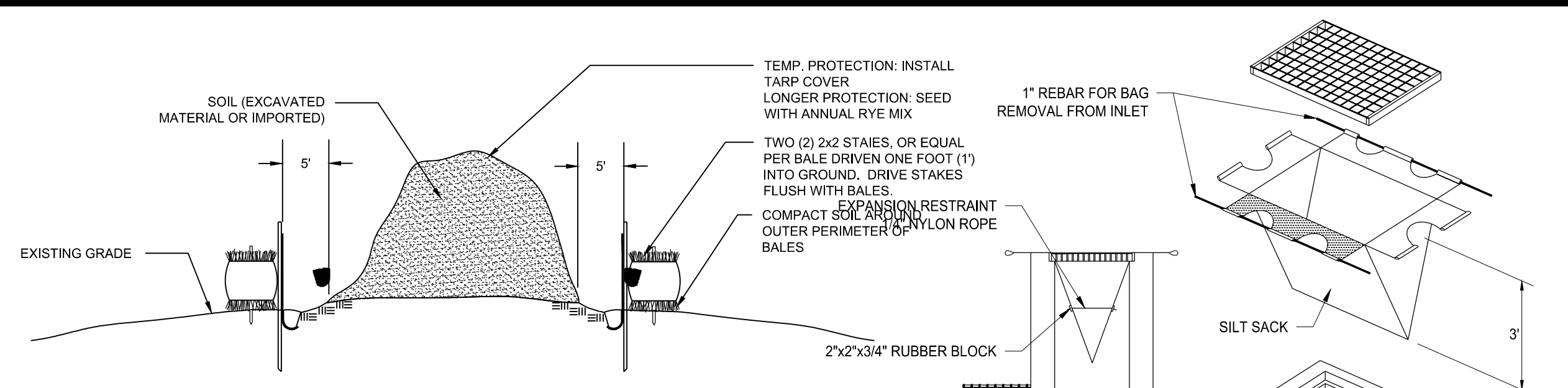
STOCKPILE PROTECTION DETAIL
