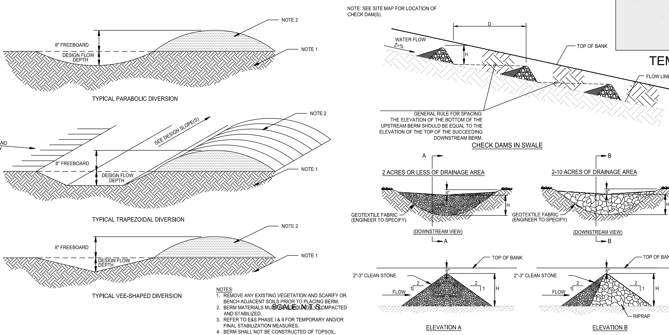
DIVERSION BERM DETAIL
