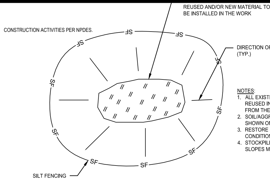
STOCKPILE AREA DETAIL
