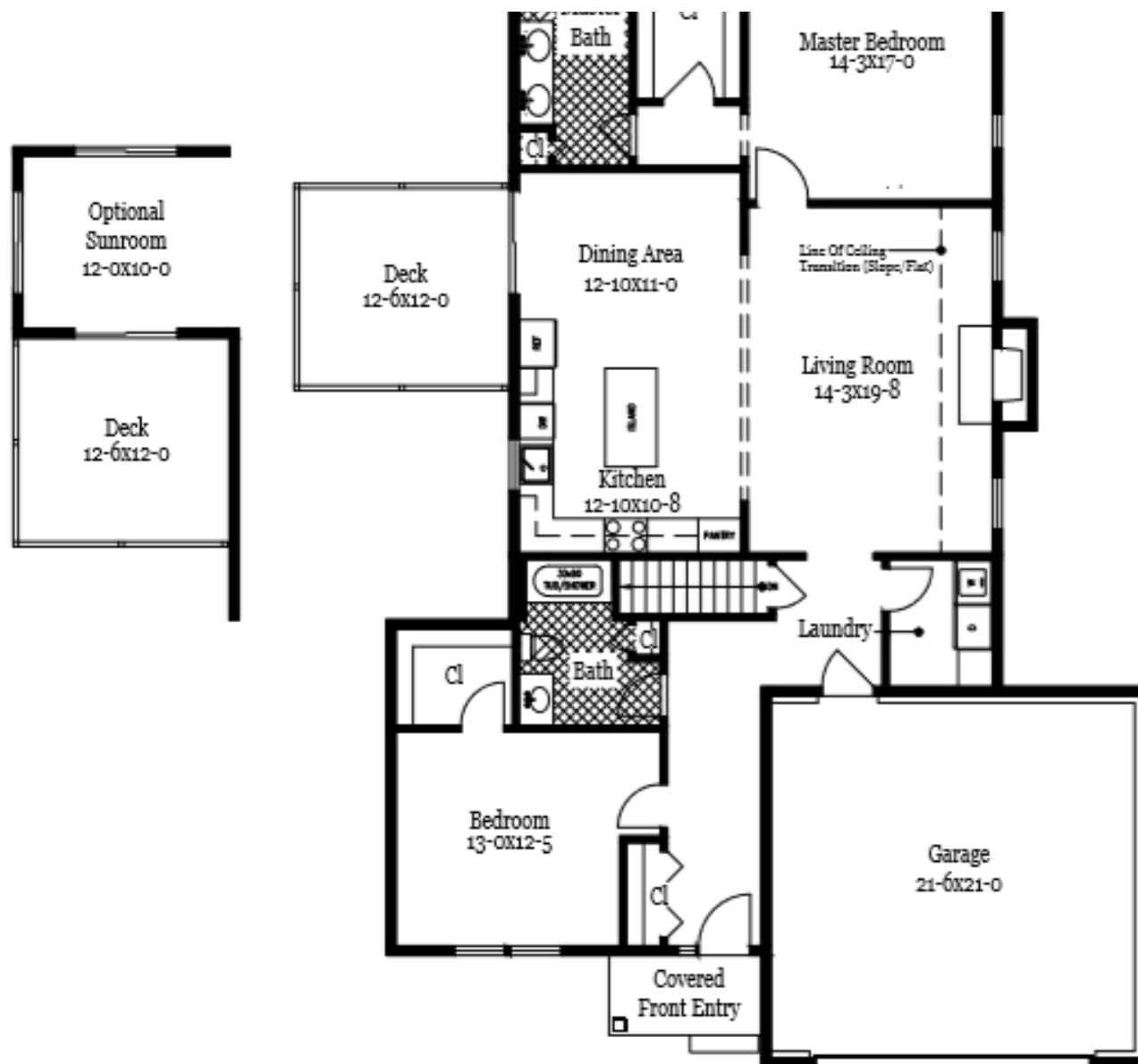
First Level Plan The Maxwell 1,700 SF 1,840 (with optional sunroom)
