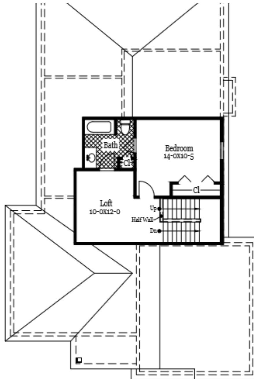
The Blake II second floor plan
