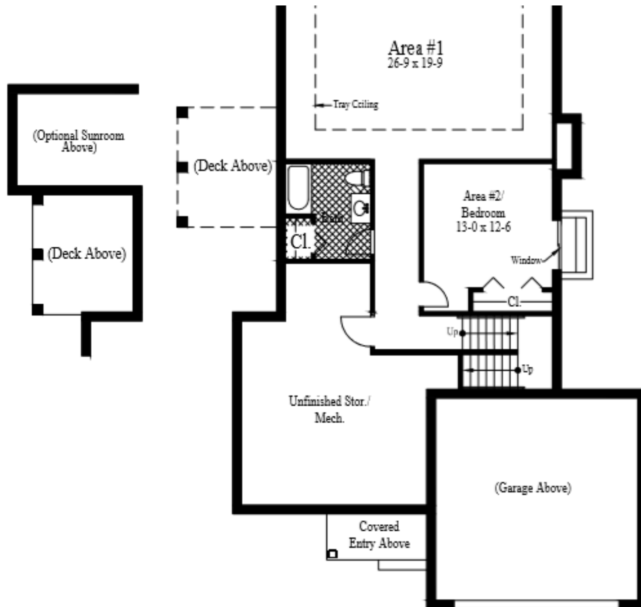
The Madison Optional Lower Level Plan 1,005 SF
